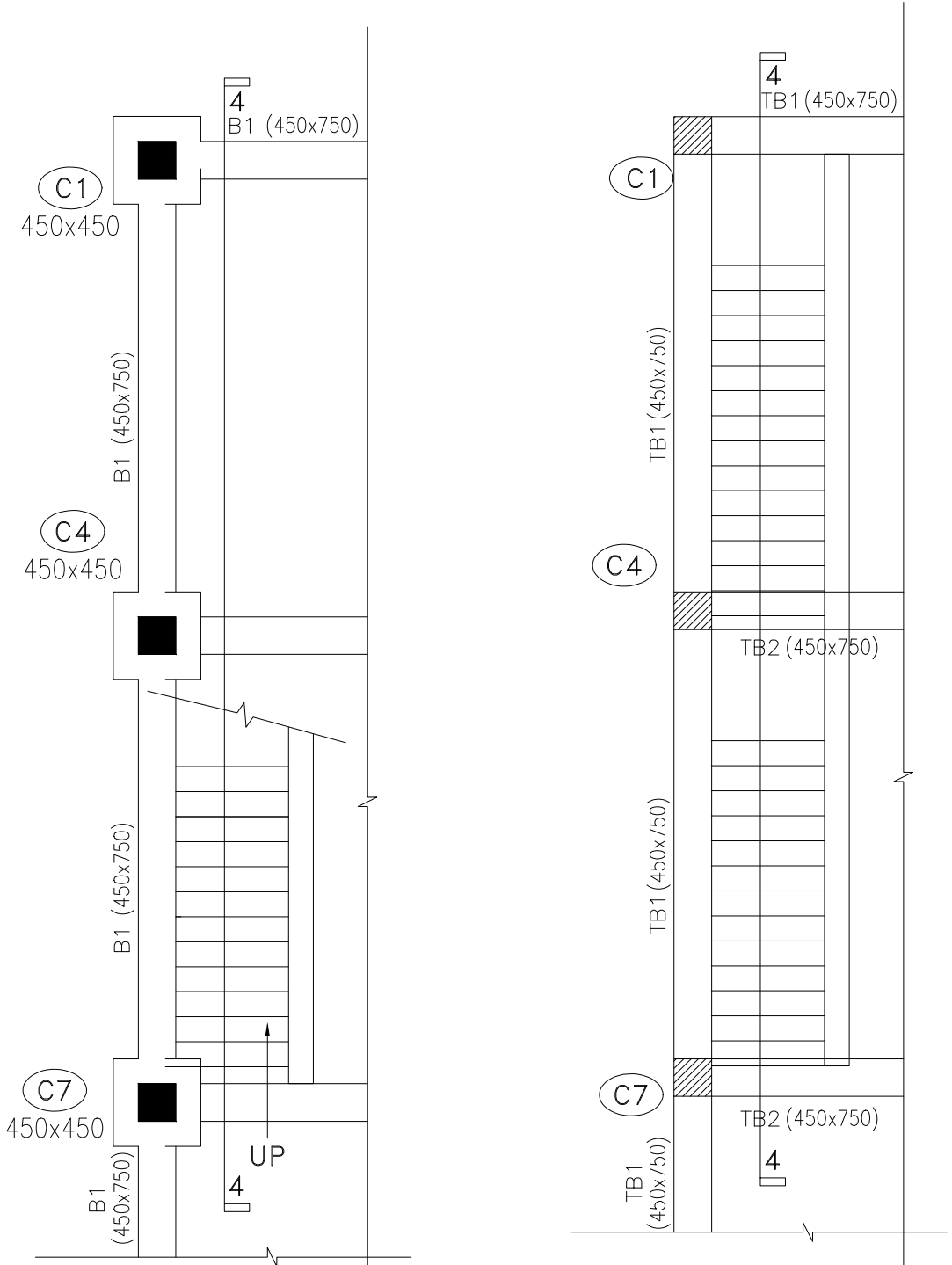
PUMP ROOM BOTTOM PLAN
