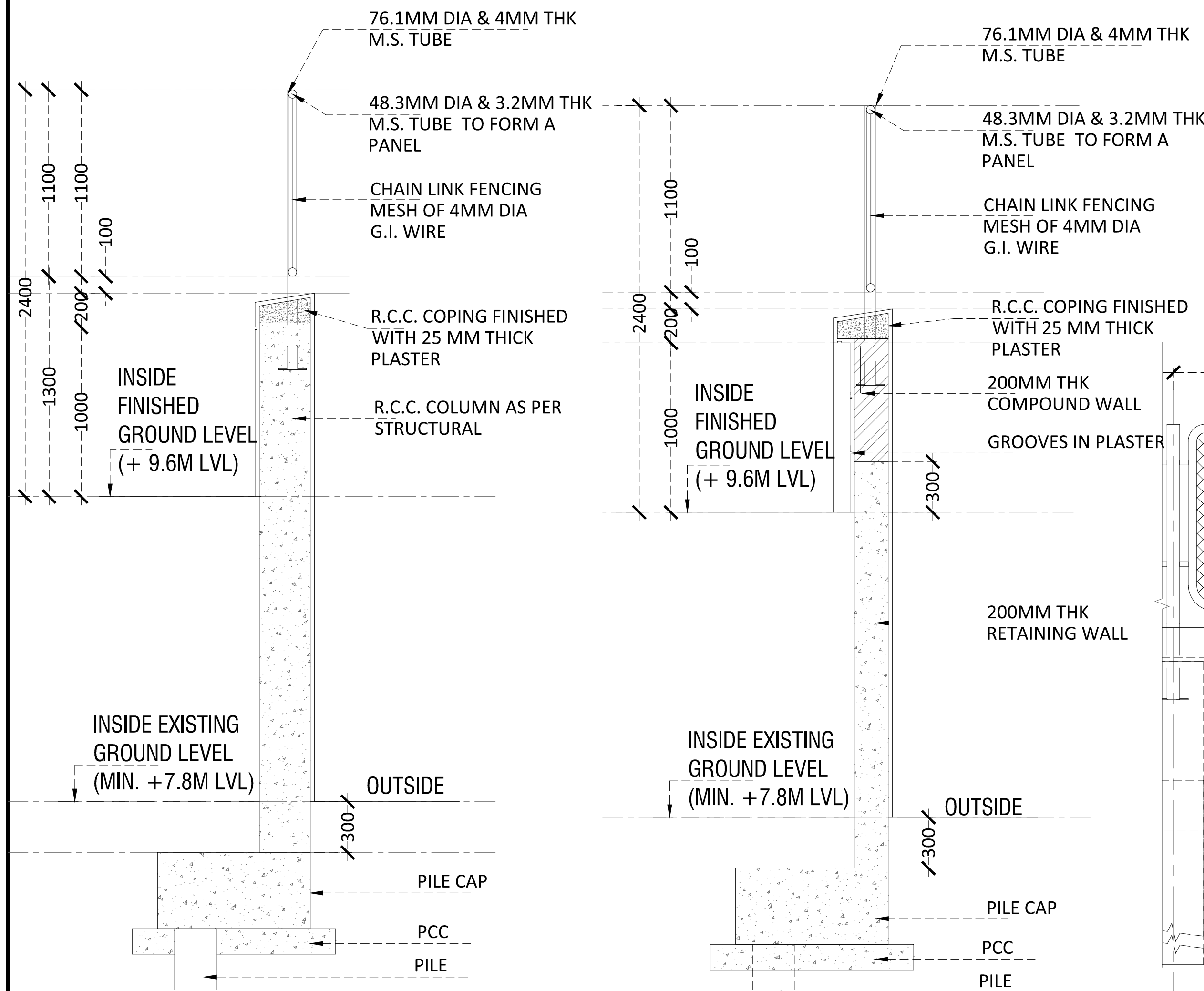
TYPICAL SECTION THROUGH COLUMN
