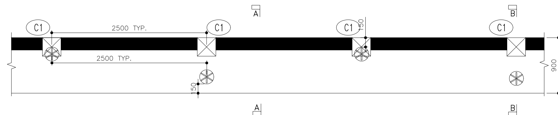
PART PLAN @ PILE FOUNDATION LAYOUT
