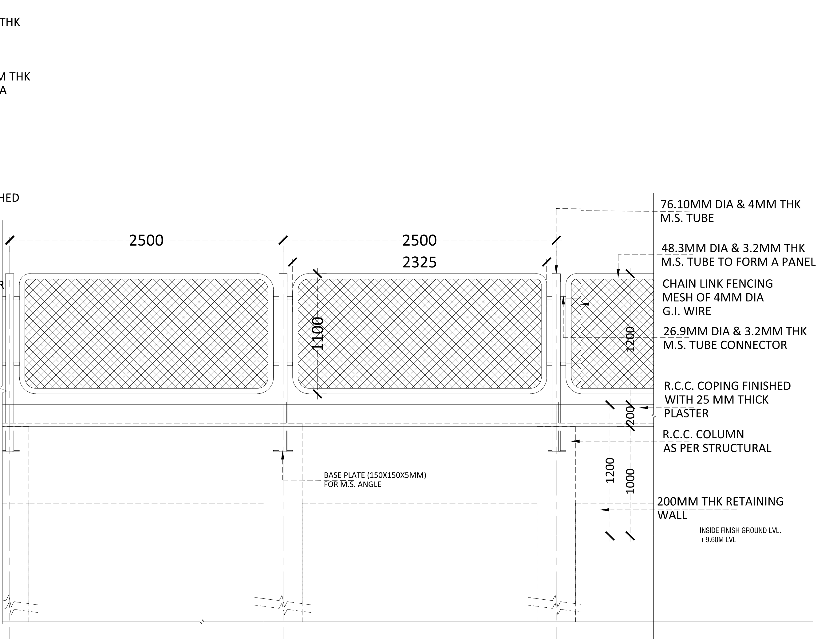
TYPICAL ELEVATION-OUTSIDE (EAST, WEST & SOUTH SIDE)
