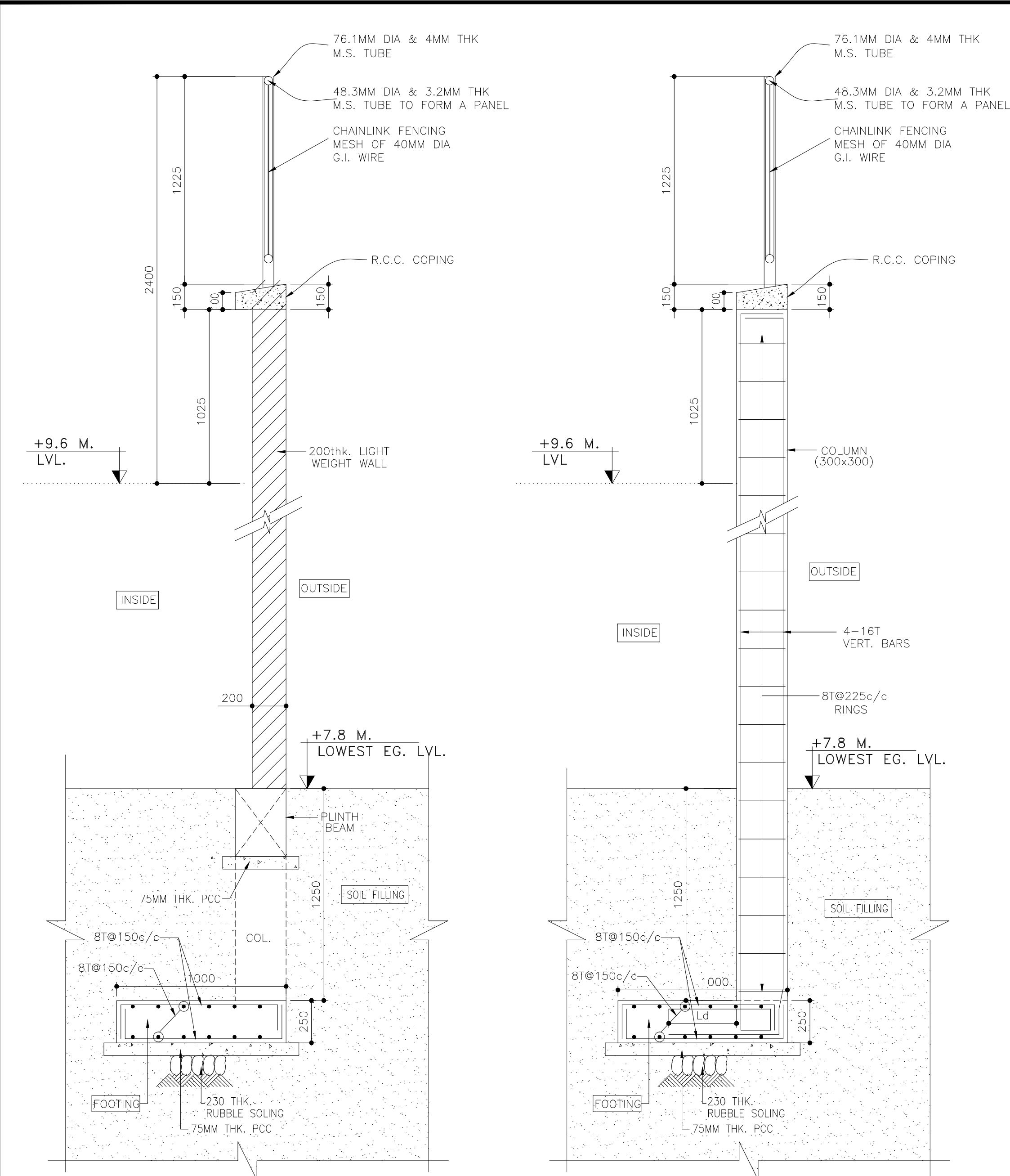
SECTION A-A TYPICAL SECTION THROUGH COMPOUND WALL
