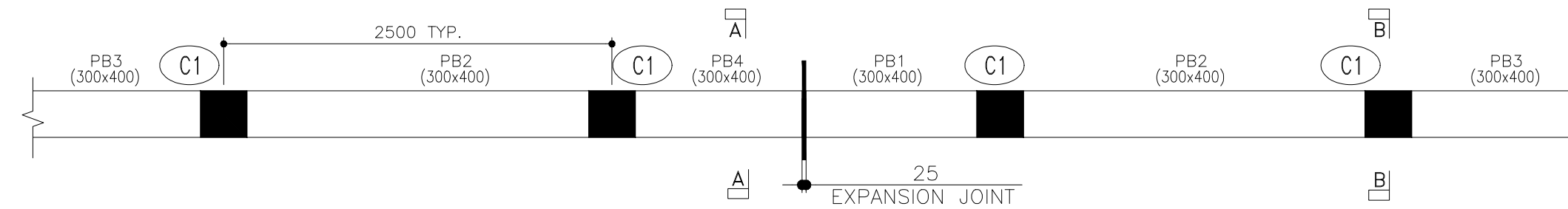
PART PLAN @ GROUND LEVEL LAYOUT
